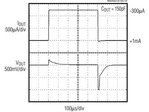
MAX6018_12 LOAD-TRANSIENT RESPONSE
