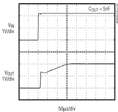
MAX6018_21 TURN-ON TRANSIENT
