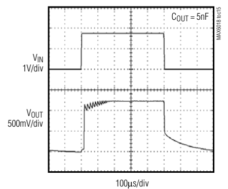
MAX6018_12 TURN-ON TRANSIENT
